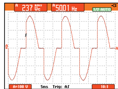
Figure 1. Thyristor voltage
