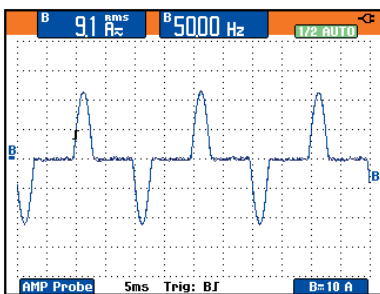
Figure 3A. Single-phase, non-linear load current waveform
