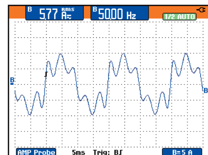
Figure 2A. Distorted current waveform
