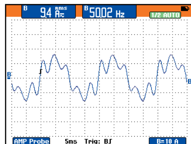
Figure 3B. Three-phase, non-linear load current waveform
