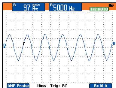
Figure 5. Neutral current
