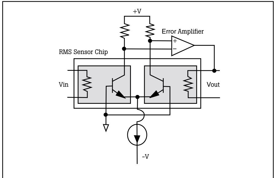
Figure 1. Simplified RMS Sensor Circuit
