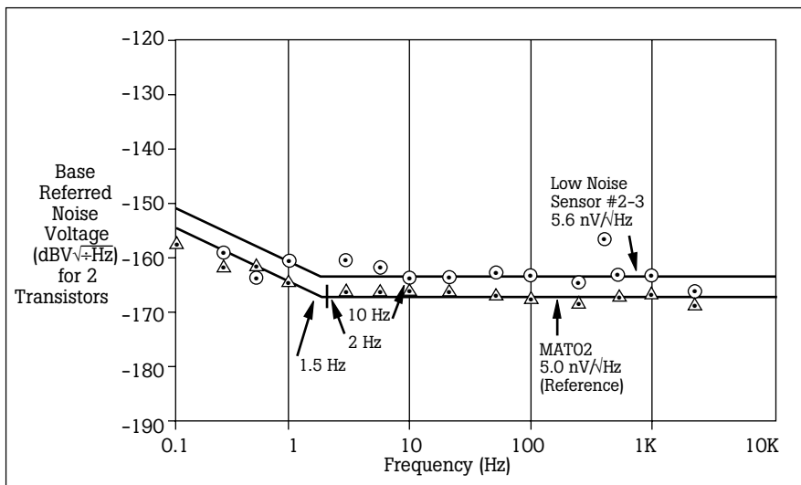
Figure 3: Base Referred Voltage Noise: Improved Sensor
