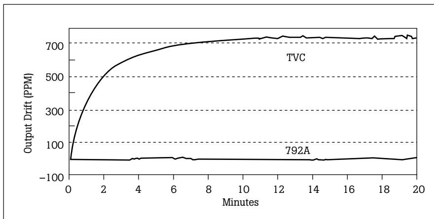
Figure 10: 792A Output Drift and Stability 2V Range
