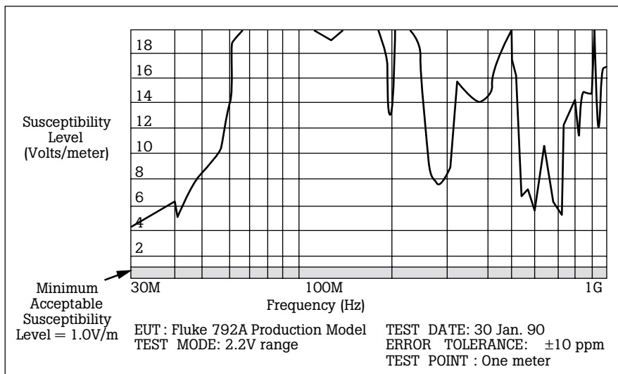
Figure 15: Radiated Susceptibility: MIL-T-28800D RS03 (Production Model)
