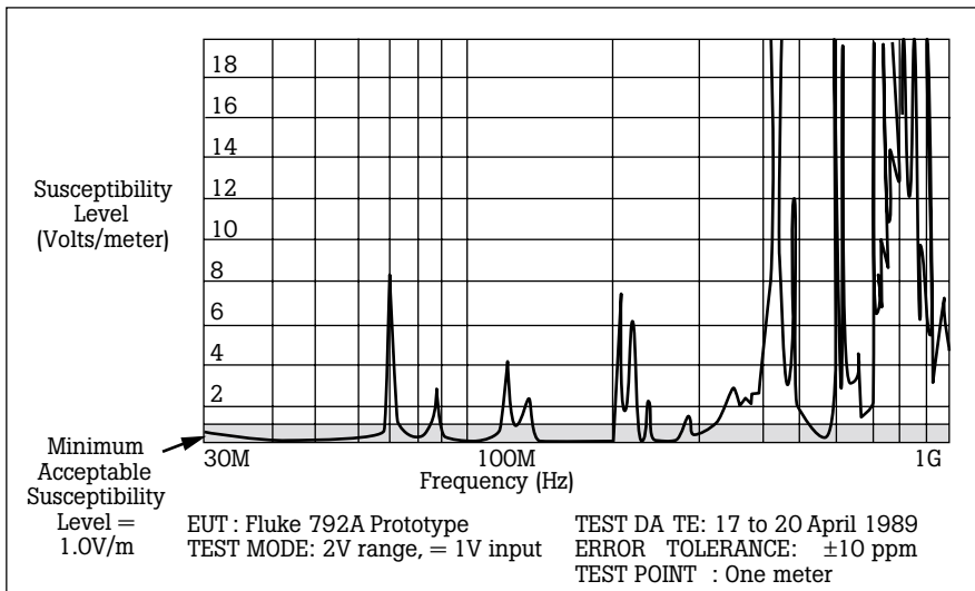
Figure 14: Radiated Susceptibility: MIL-T-28800D RS03 (Design Model)
