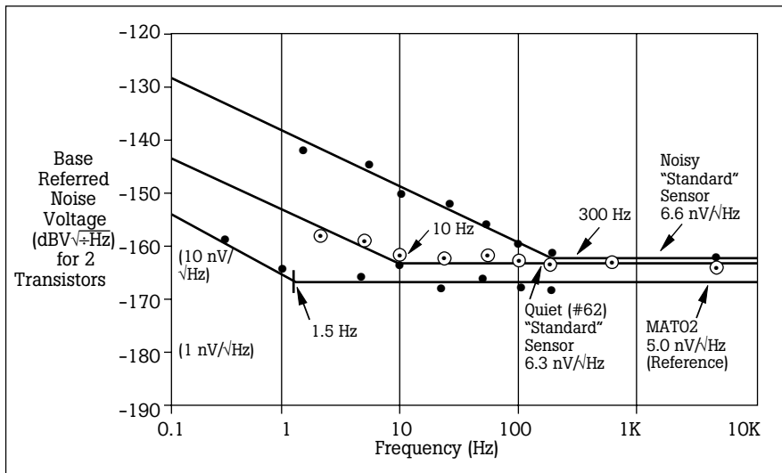
Figure 2: Base Referred Voltage Noise: Original Sensor
