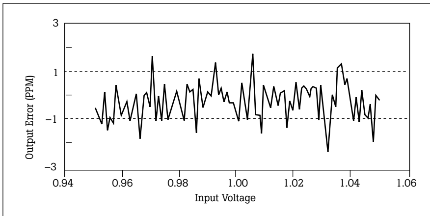
Figure 9: Linearity Error in 792A 2V Range: 0.95 to 1.05 Volts
