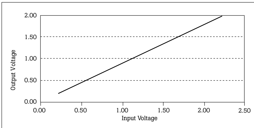
Figure 8: Linearity of 792A 2V Range: 0.22 to 2.2 Volts
