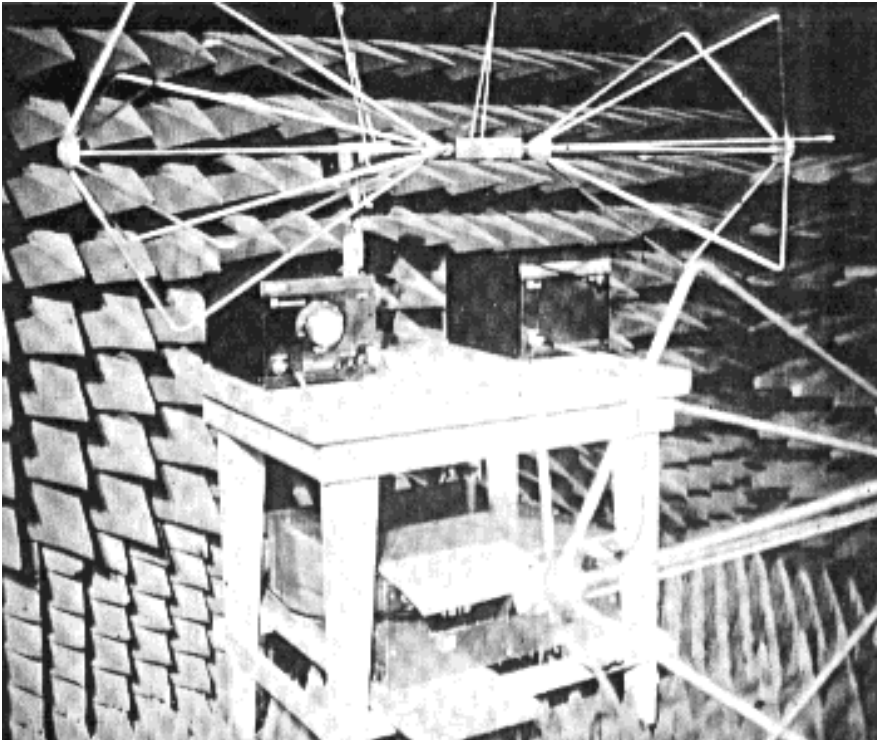
Figure 13: Electromagnetic Interference Immunity Test Setup.
