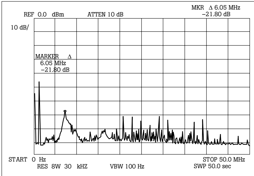
Figure 7: Spectrum of a Calibrator Output at 1 mV, 1 MHz
