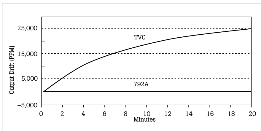
Figure 11: Output Drift and Stability 1000V Range
