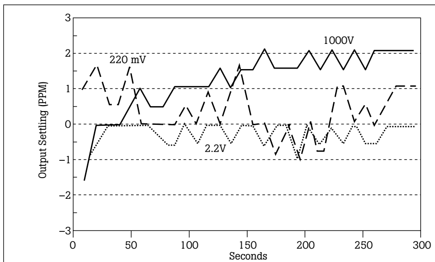
Figure 12: 792A Output Settling: 220 mV, 2V Ranges
