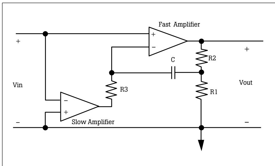
Figure 6: Noninverting Composite Amplifier
