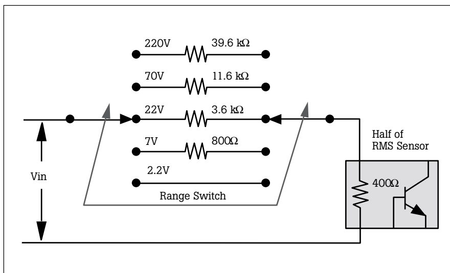
Figure 5: Simplified 792A Passive Range
