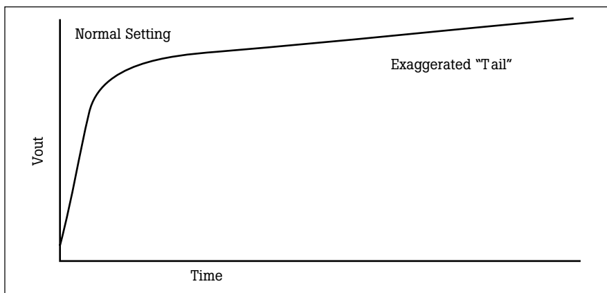
Figure 4: RMS Sensor Output Settling Before Thermal Improvements
